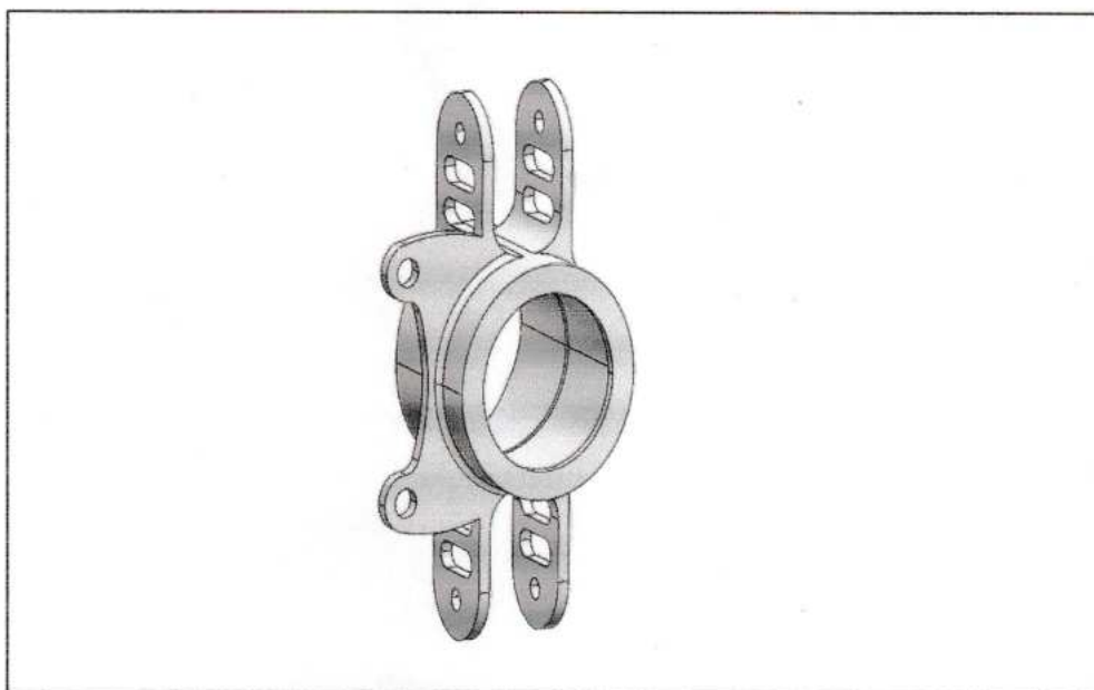
PERSPECTIVE VIEW
